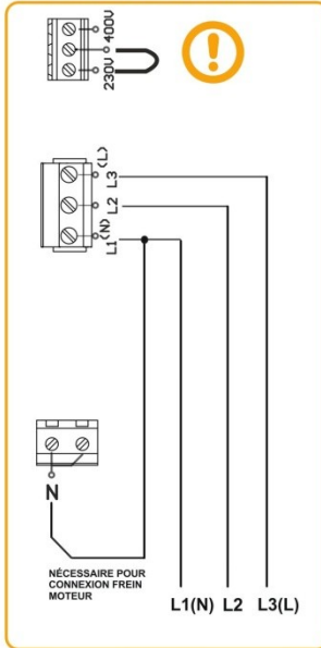
ALIMENTATION 230V TRIPHASE
