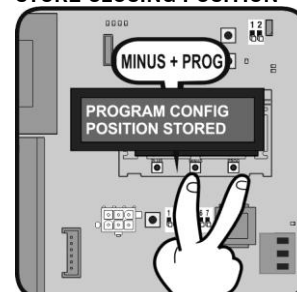
PRESS MINUS + PROG TO STORE CLOSING POSITION
